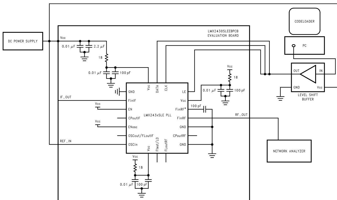
Figure 27. Input Impedance Test Setup
