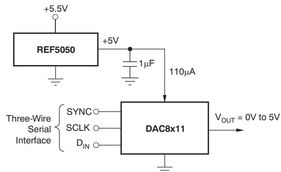
Figure 88. REF5050 as Power Supply to DAC8x11
