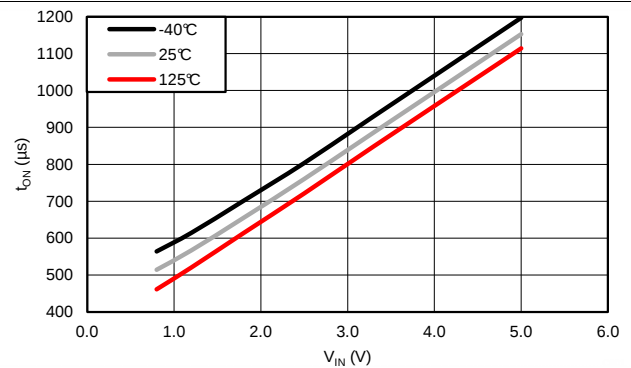
Figure 20. t_{ON} vs V_{IN} , V_{BIAS} = 5 V
