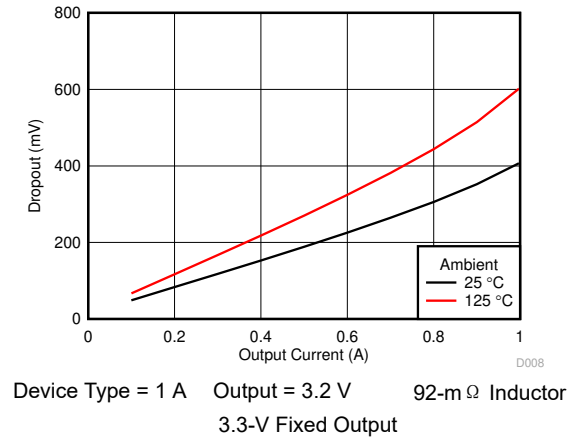
图 9-16. Dropout Voltage
