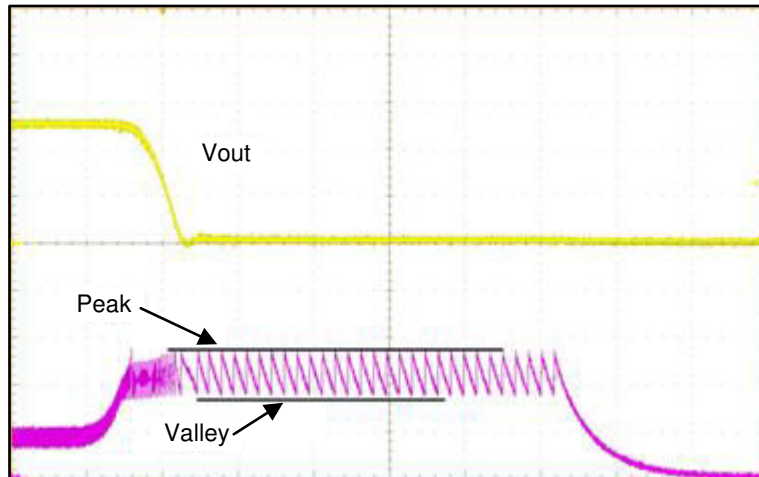
图 8-3. Current Limit Operation
