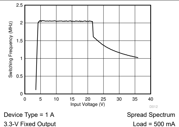
图 9-18. Frequency vs. Input Voltage
