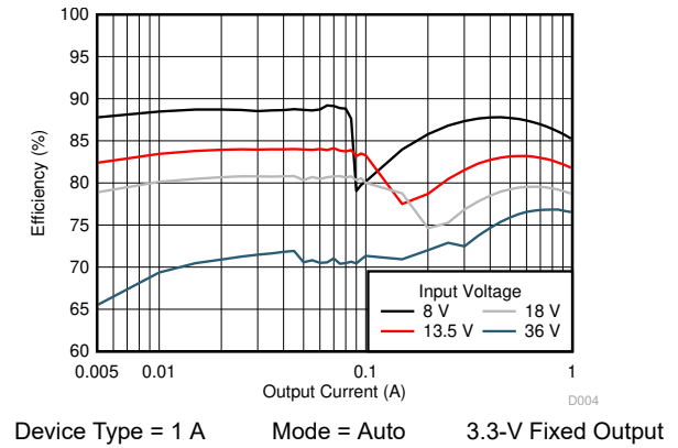
图 9-14. Efficiency
