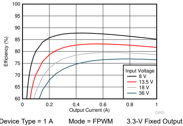
图 9-13. Efficiency
