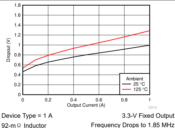
图 9-17. Entry into Dropout
