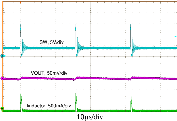
图 8-8. Typical PFM Switching Waveforms
