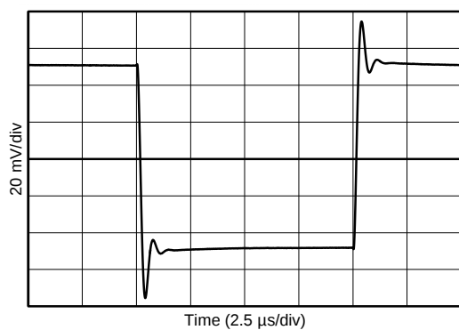
Figure 23. Overload Recovery
