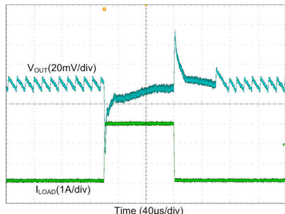
图 8-18. Buck Transient Load Step Response, Forced-PWM Mode
