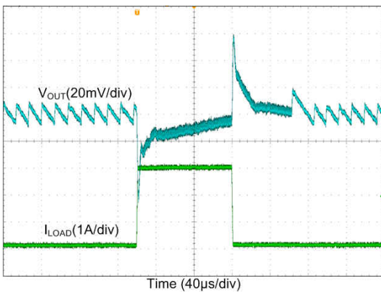
图 8-17. Buck Transient Load Step Response, Forced-PWM Mode
