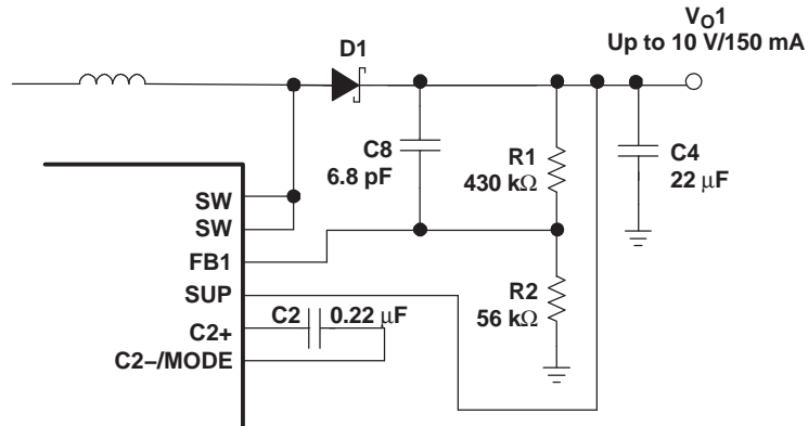
Figure 2. Feed-forward Capacitor
