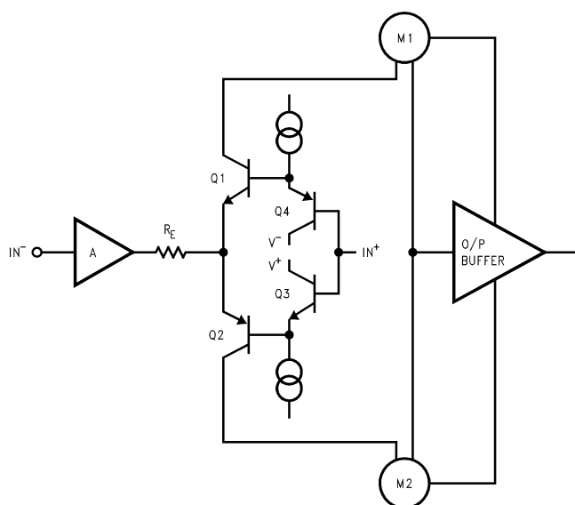
Simplified Schematic Diagram
