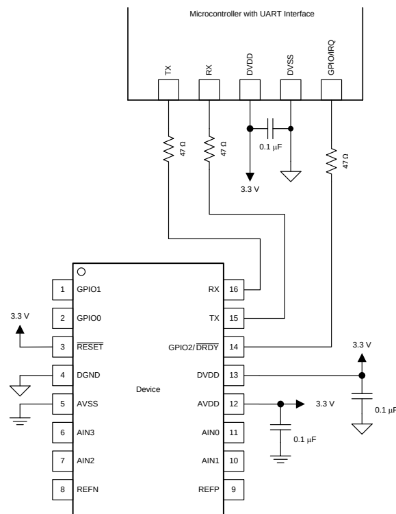
图 74. Interface Connections
