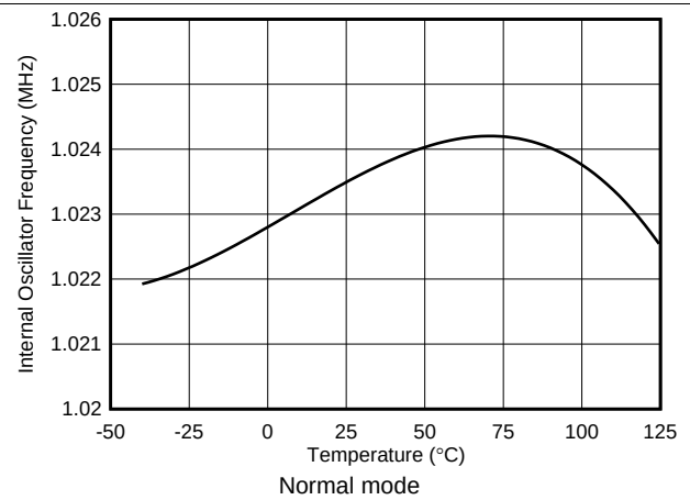
图 31. Internal Oscillator Frequency vs Temperature
