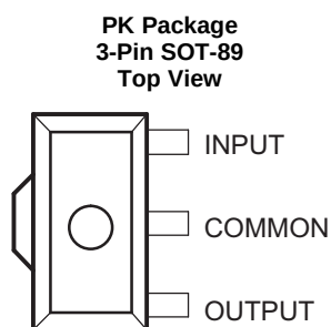
Pin Functions
