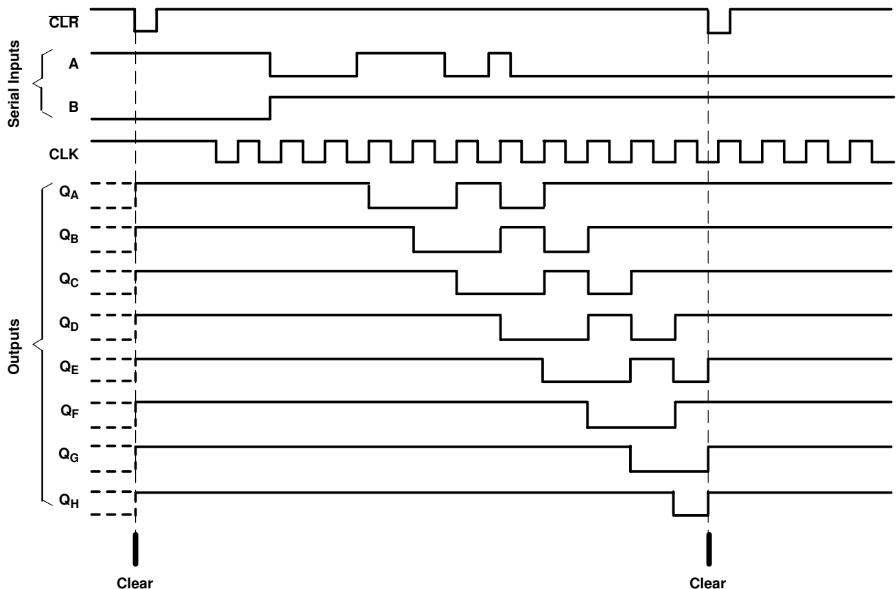
Figure 9-2. Application timing diagram
