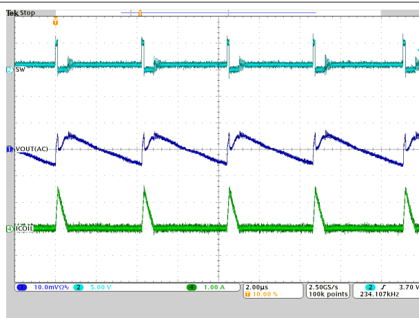
图 9-15. Switching Frequency
