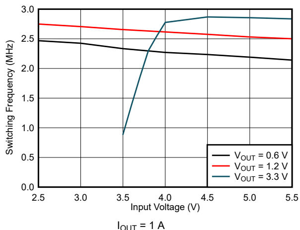
图 9-15. Switching Frequency
