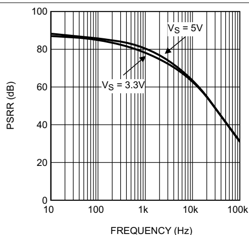
Figure 8. PSRR vs Frequency
