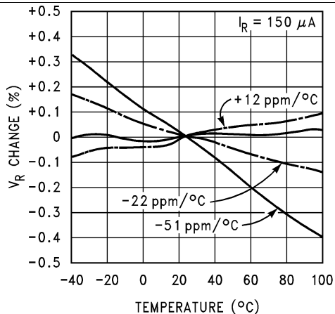
Figure 1. Temperature Drift For Different Average Temperature Coefficient
