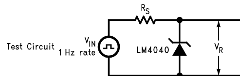
Figure 9. Test Circuit
