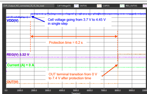
Figure 9-4. Overvoltage Protection
