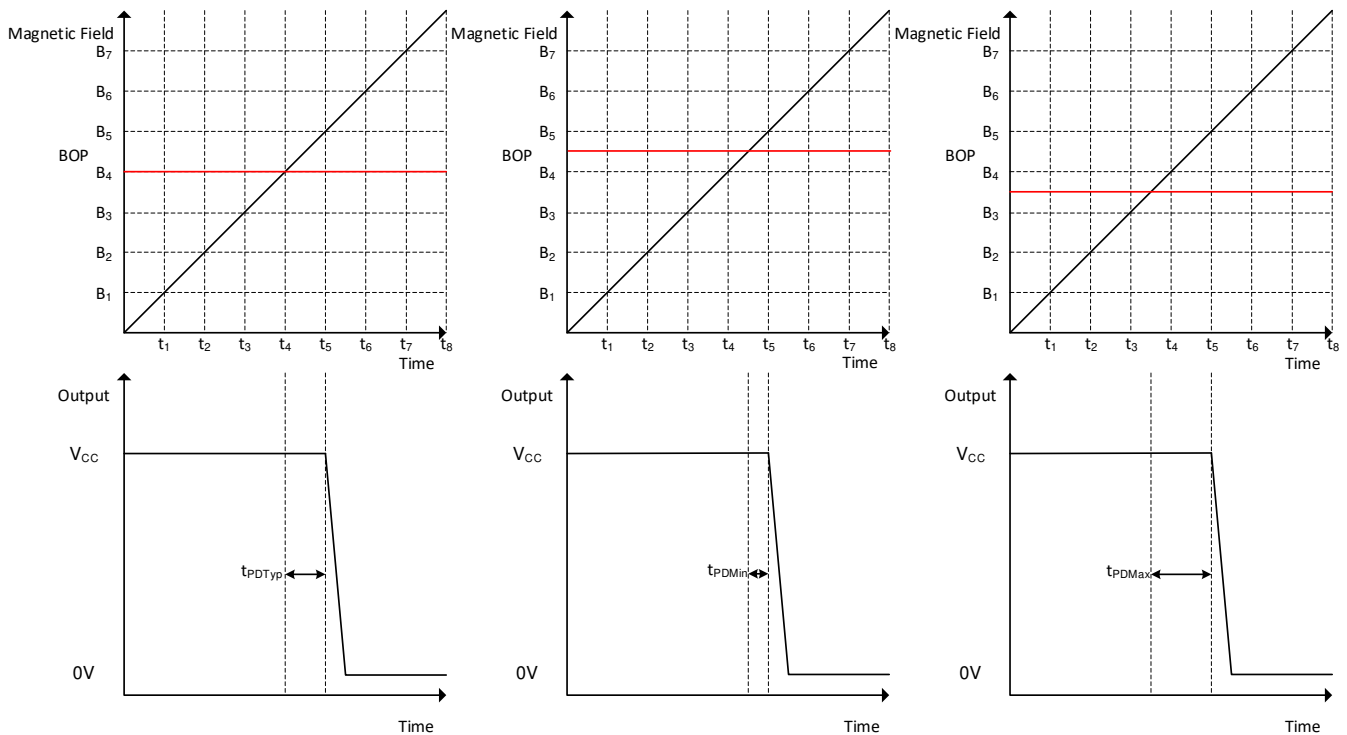
图 8-19. Field Sampling Timing
