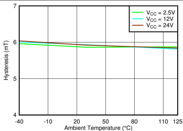
图 7-44. Hysteresis_Z vs. Temperature
