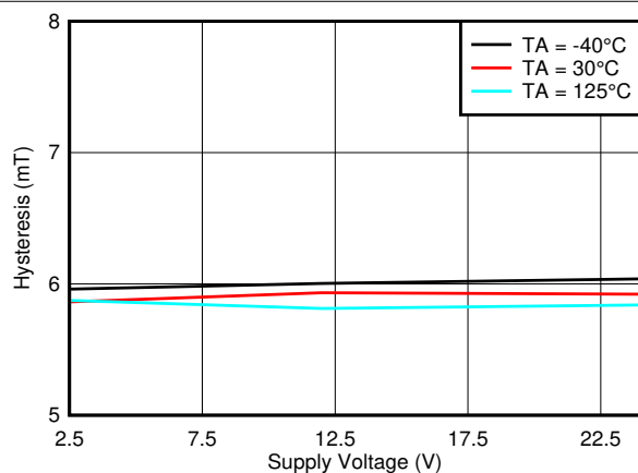
图 7-43. Hysteresis_Z vs. VCC
