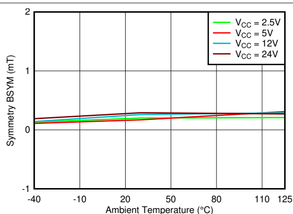
图 7-24. B_{SYM(y)} vs. Temperature
