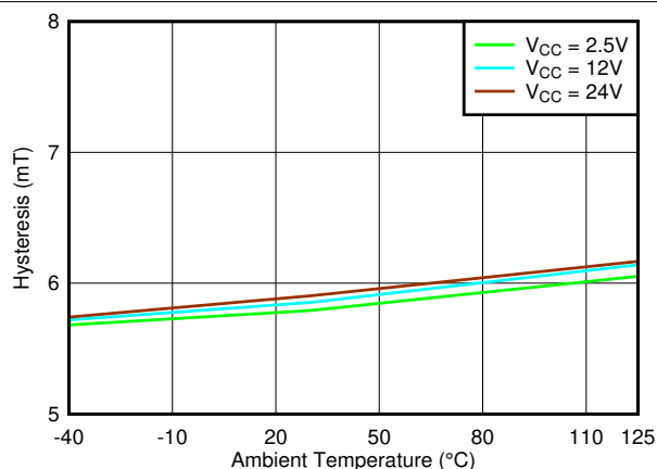
图 7-50. Hysteresis_X vs. Temperature
