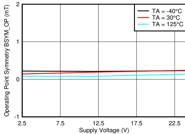
图 7-71. B_{SYM\_OP(XY)} vs. V_{CC}
