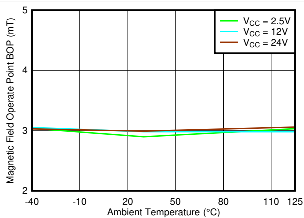
图 7-40. BOP_Z Threshold vs. Temperature
