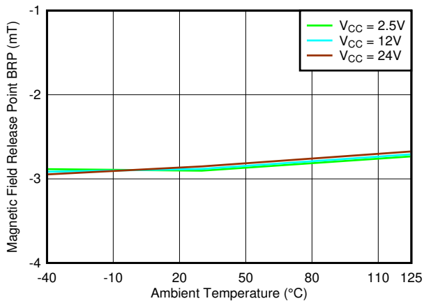
图 7-42. BRP_Z Threshold vs. Temperature
