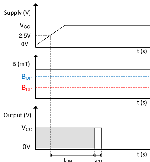
图 8-18. Power-On Time When B > B_{OP}
