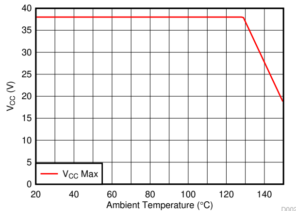
图 8-22. Power Derating Curve
