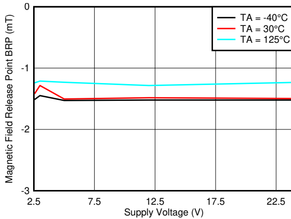
图 7-15. B RP_Y Threshold vs. V CC
