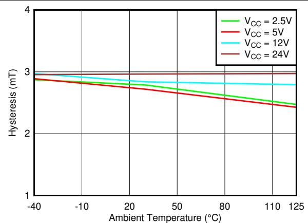
图 7-12. Hysteresis_X vs. Temperature
