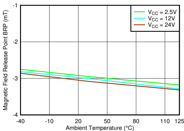
图 7-48. B RP_X Threshold vs. Temperature
