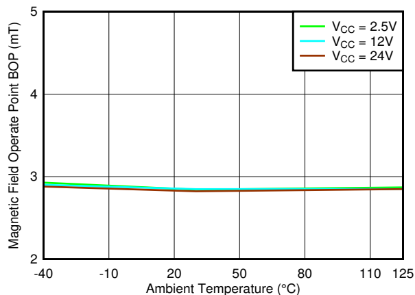
图 7-46. B OP_X Threshold vs. Temperature
