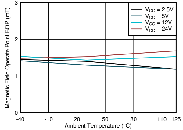
图 7-8. B_{OP\_X} Threshold vs. Temperature
