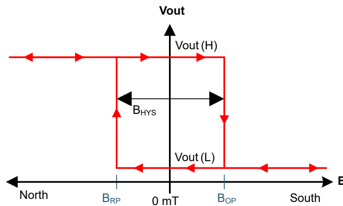
图 8-2. Latch Functionality
