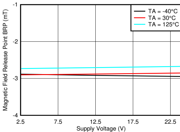
图 7-41. BRP_Z Threshold vs. VCC
