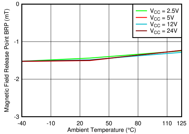
图 7-16. B RP_Y Threshold vs. Temperature
