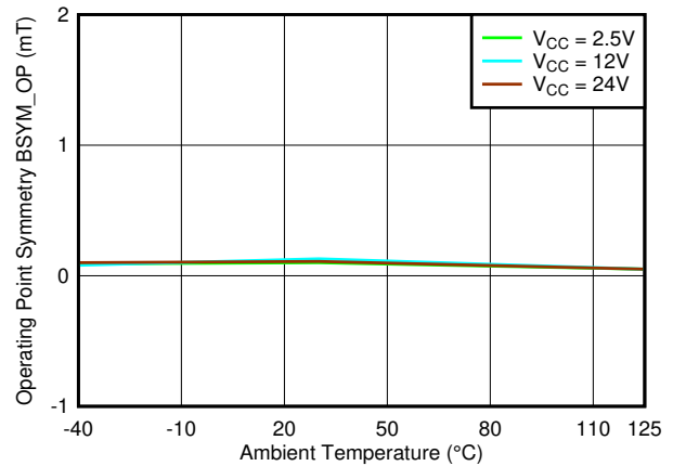
图 7-72. B_{SYM\_OP(XY)} vs. Temperature
