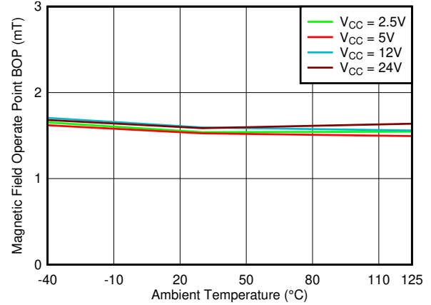
图 7-14. B OP_Y Threshold vs. Temperature
