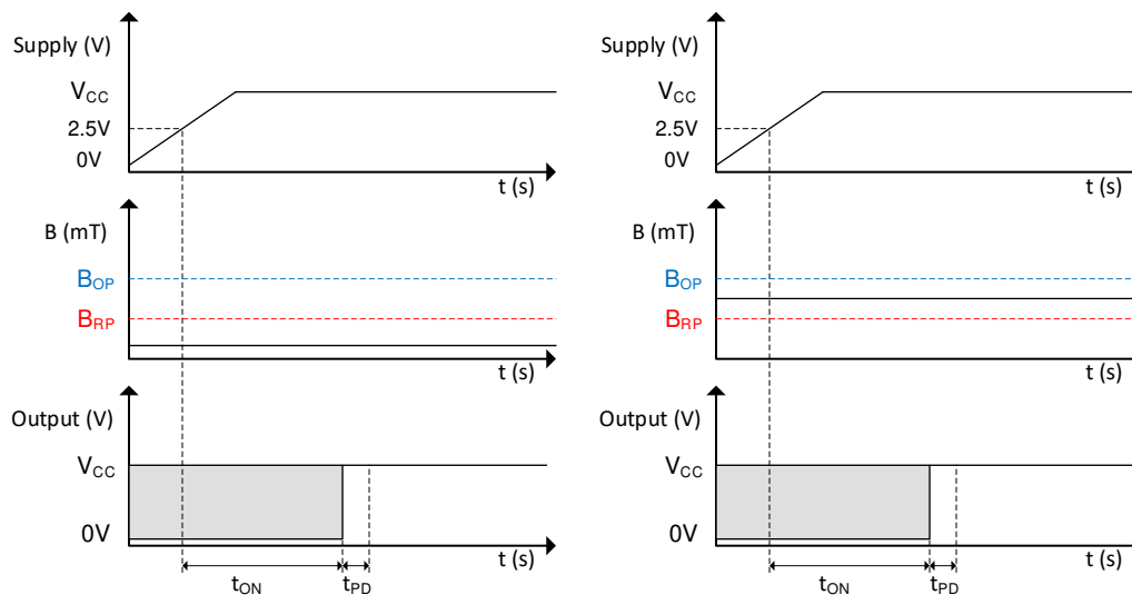
图 8-17. Power-On Time When B < B_{OP}
