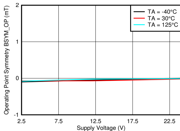
图 7-33. B_{SYM\_OP(XY)} vs. V_{CC}
