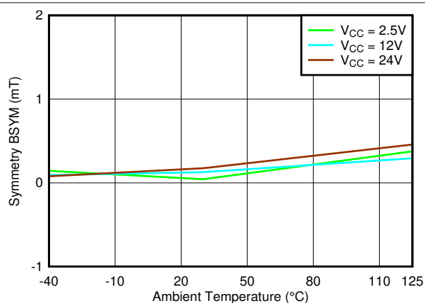
图 7-58. B_{SYM(Z)} vs. Temperature
