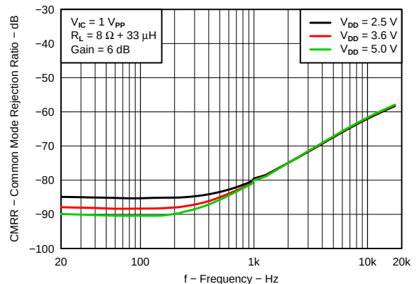
Figure 24. Common Mode Rejection Ratio vs Frequency
