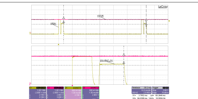
Figure 36. Boost Charger Operational Waveforms
