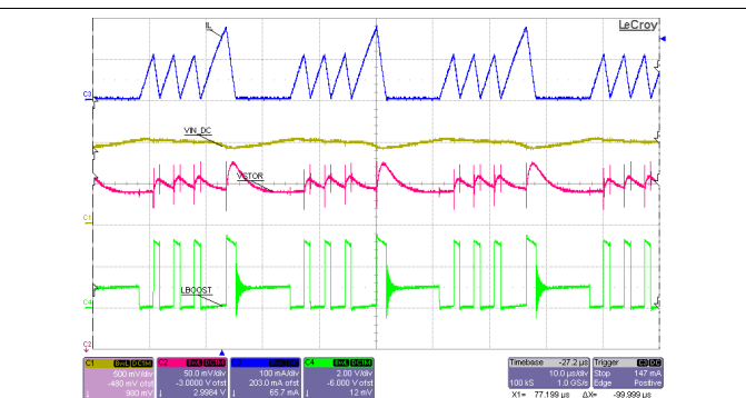
V_{IN\_DC} = sourcemeter with V_{SOURCE} = 2.0\text{ V} and compliance of 43 mA V_{BAT\_SEC} = sourcemeter with V_{SOURCE} = 3.0\text{ V} and compliance of 1 A I_L = inductor current
