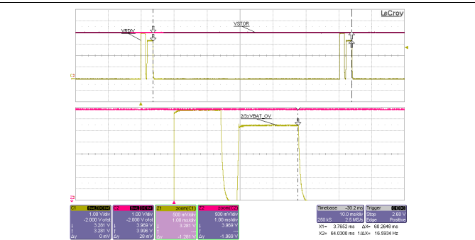
VIN_DC = sourcemeter with V_{SOURCE} = 2.0 V and compliance of 43 mA VBAT_SEC = sourcemeter with V_{SOURCE} = 4.0 V and compliance of 1 A
