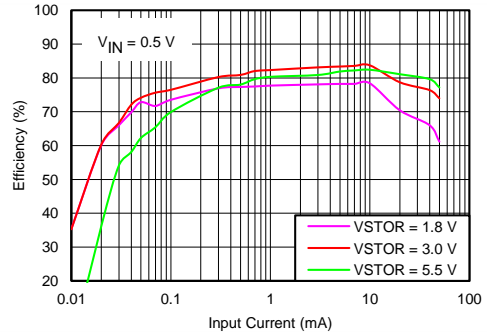
VIN_DC = Keithley Source Meter configured with voltage source = 0.5 V and I COMP varied from 0.01 mA to 100 mA VSTOR = Keithley Sourcemeter configured to measure current and voltage source set to hold the VSTOR voltage = 1.8 V, 3.0 V or 5.5 V
