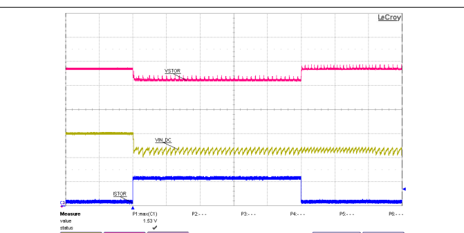
V_{IN\_DC} = 1.5\text{ V} with 75\ \Omega series resistance V_{BAT} = 4.2\text{ V} charged 0.5 F capacitor R(V_{STOR}) = open to 84\ \Omega to open
