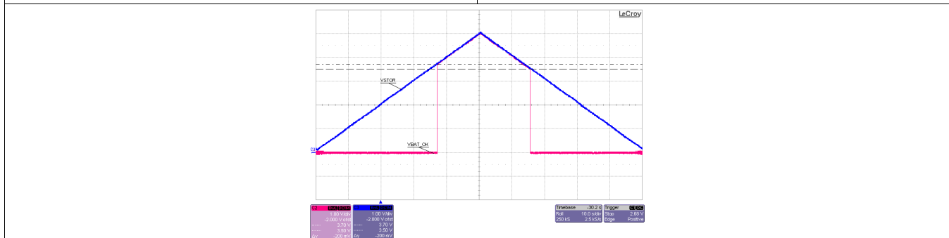
VIN_DC floating No storage element on VBAT or VBAT_PRI VSTOR artificially ramped from 0 V to 5 V to 0 V using a function generator
