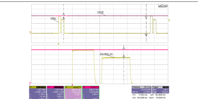
V_{IN\_DC} = sourcemeter with V_{SOURCE} = 2.0\text{ V} and compliance of 43 mA V_{BAT\_SEC} = sourcemeter with V_{SOURCE} = 3.6\text{ V} and compliance of 1 A
