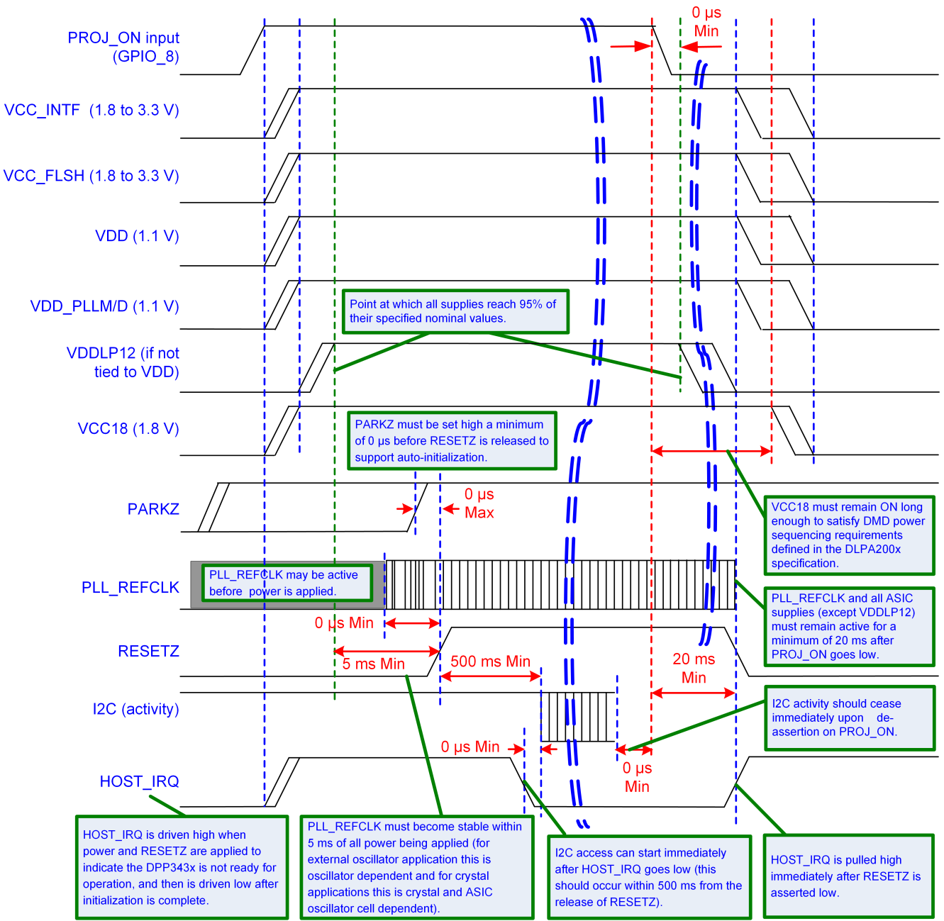
Figure 27. DLPC343x Power-Up / PROJ_ON = 0 Initiated Normal PARK and Power-Down
