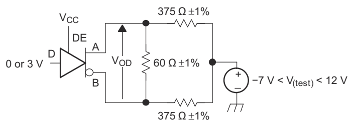
Figure 8-2. Driver V_{OD} With Common-Mode Loading Test Circuit
