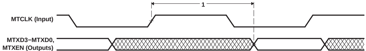
Figure 6-47. EMAC Transmit Interface Timing
