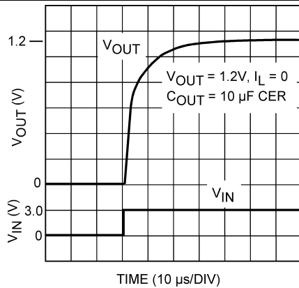
Figure 26. Turnon Time
