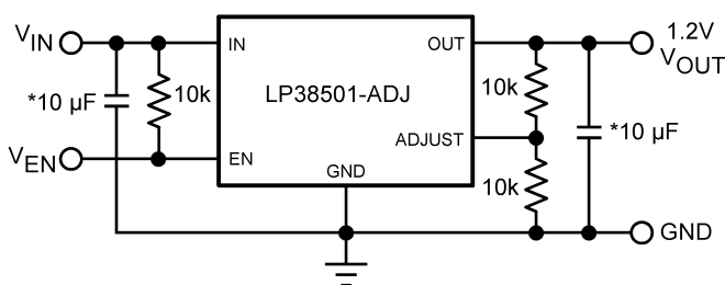
Figure 23. Typical Circuit (LP38501)
