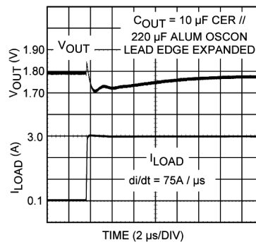
Figure 22. 10-µF Ceramic Paralleled by 220-µF OSCON
