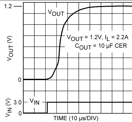
Figure 27. Turnon Time
