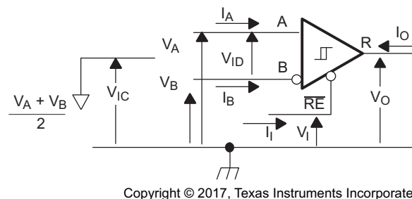
Figure 24. Receiver Voltage and Current Definitions
