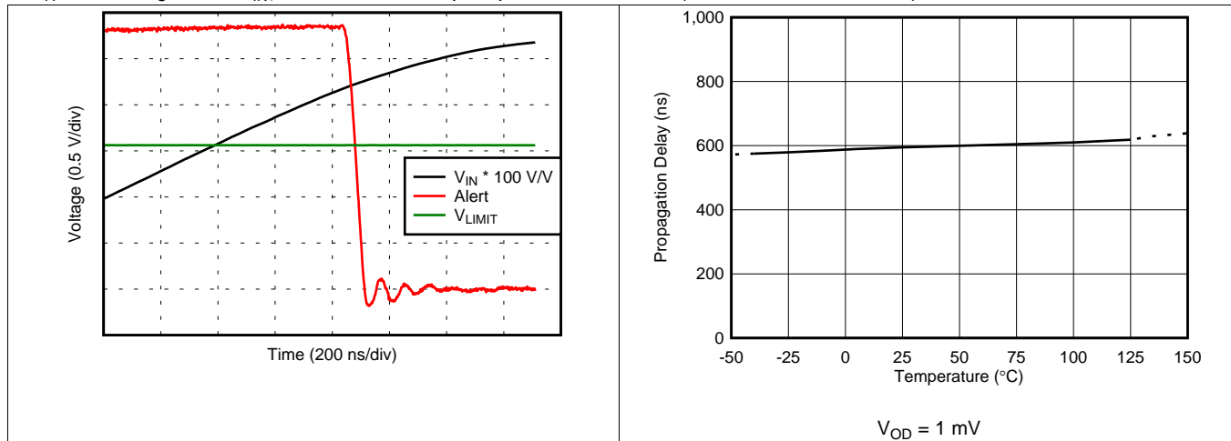
图 32. Comparator Propagation Delay vs Temperature
