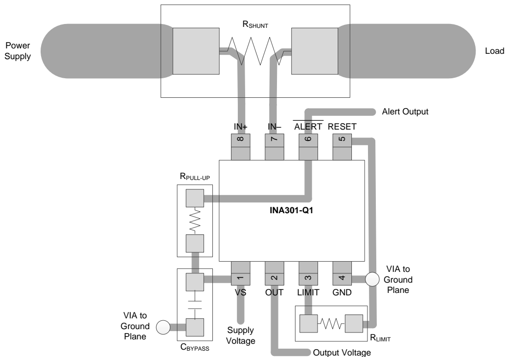
图 44. Recommended Layout
