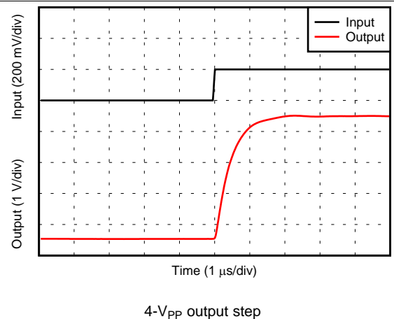
图 24. Voltage Output Rising Step Response
