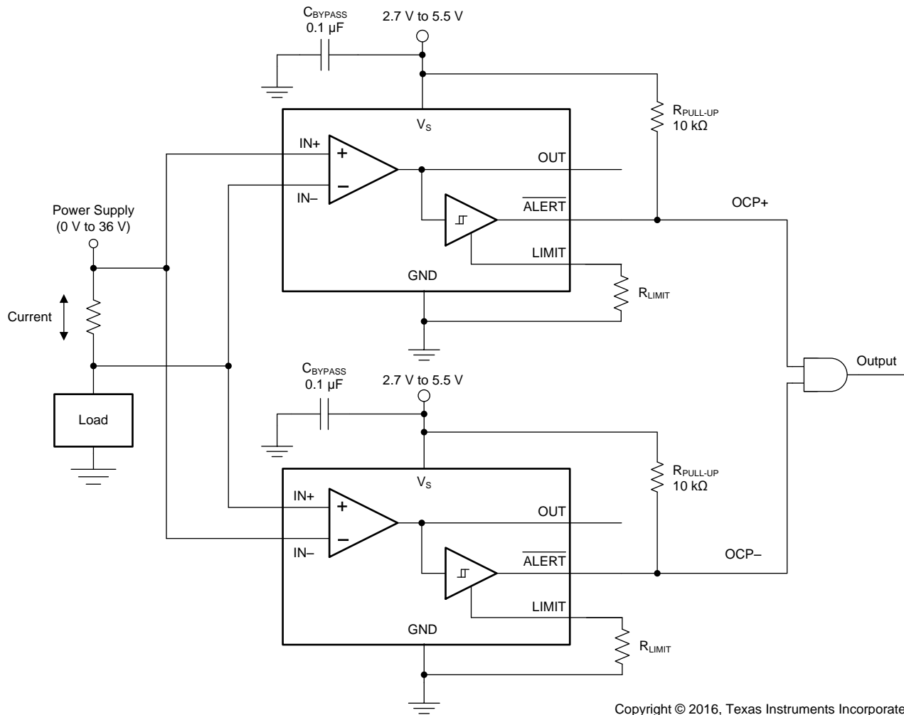
图 42. Bidirectional Application
