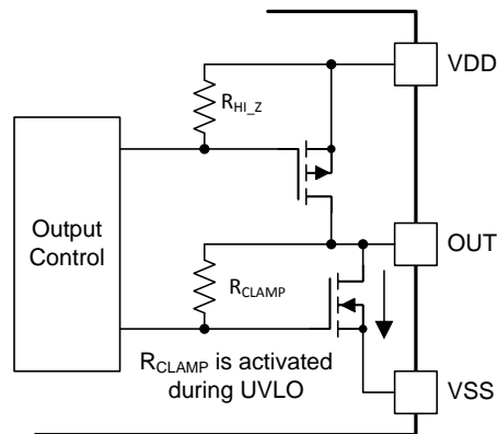
图 31. Simplified Representation of Active Pull Down Feature
