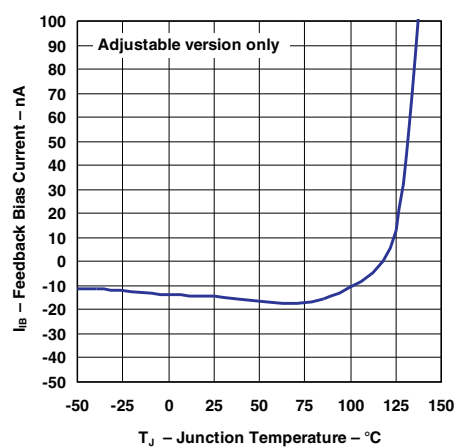
Figure 10. FEEDBACK Current
