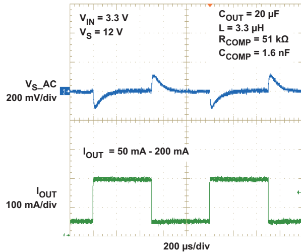
Figure 11. Load Transient Response High Frequency (1.2 MHz)
