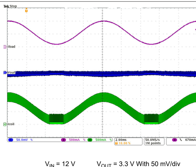
图 9-30. PWM-PSM-Transition
