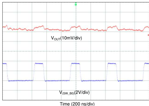
Figure 82. Output Voltage Ripple, Forced-PWM Mode (3-Phase Output)
