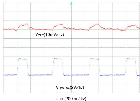
Figure 84. Output Voltage Ripple, Forced-PWM Mode (1-Phase Output)
