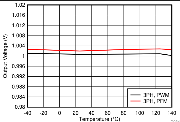
Figure 59. Output Voltage vs Temperature (3-Phase Output)
