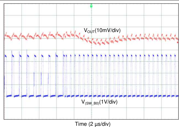
Figure 84. Output Voltage Ripple, Forced-PWM Mode (1-Phase Output)
