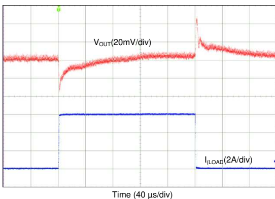
Figure 102. Transient Load Step Response, AUTO Mode (1-Phase Output)
