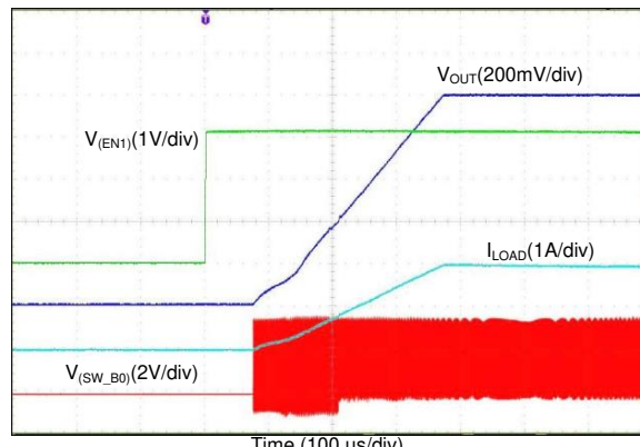
Figure 71. Start-Up With EN1, Forced PWM (2-Phase Output)
