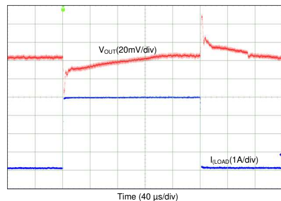
Figure 103. Transient Load Step Response, Forced-PWM Mode (4-Phase Output)
