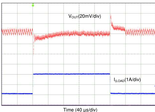
Figure 100. Transient Load Step Response, AUTO Mode (3-Phase Output)
