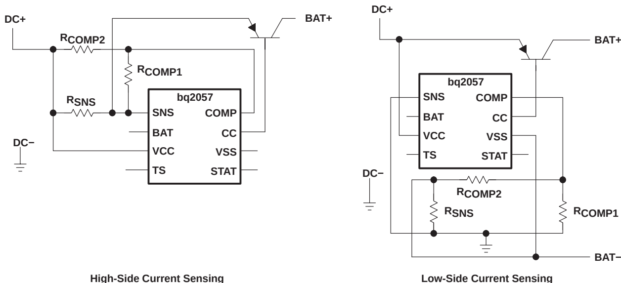
Figure 13. AutoComp Circuits
