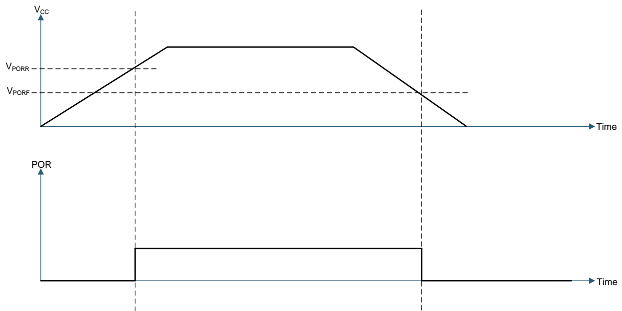
Figure 40. V_{POR}
