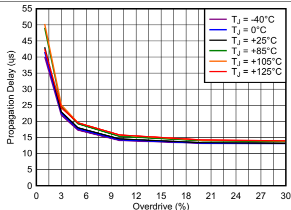
Figure 17. Propagation Delay vs Overdrive (V+ = 5.5 V)
