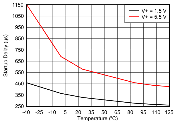
Figure 15. Startup Delay
