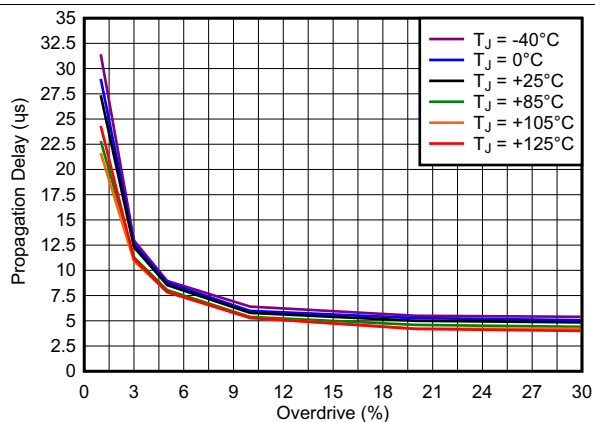
Figure 17. Propagation Delay vs Overdrive (V+ = 5.5 V)
