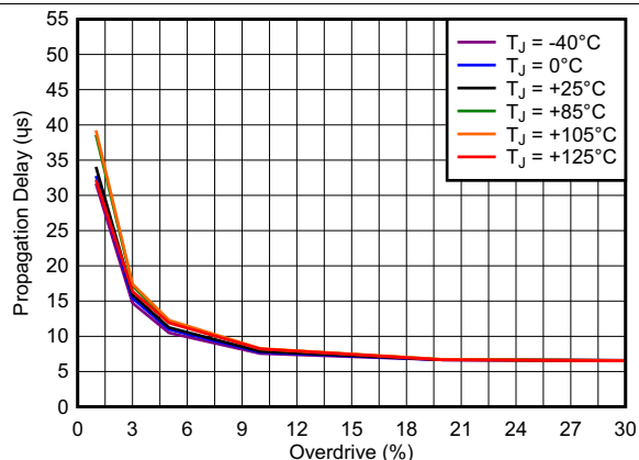
Figure 14. Propagation Delay from INx Low to Output Low
