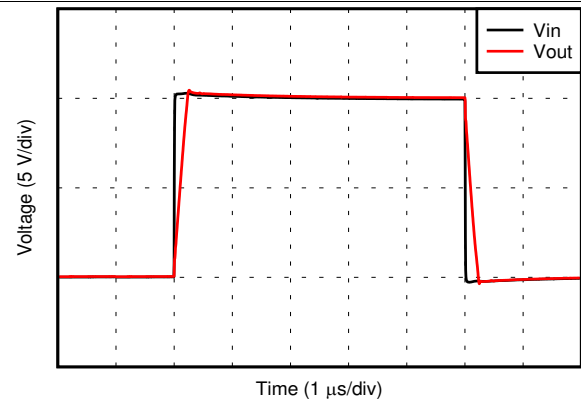
图 34. Small-Signal Step Response (Noninverting)
