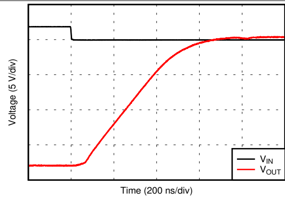
图 32. Negative Overload Recovery
