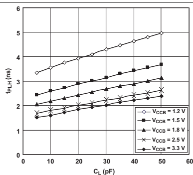
Figure 1. Typical A-to-B Propagation Delay, Low to High
