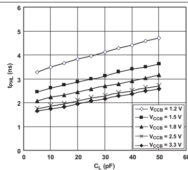
Figure 2. Typical A-to-B Propagation Delay, High to Low
