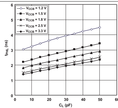
Figure 4. Typical A-to-B Propagation Delay, High to Low
