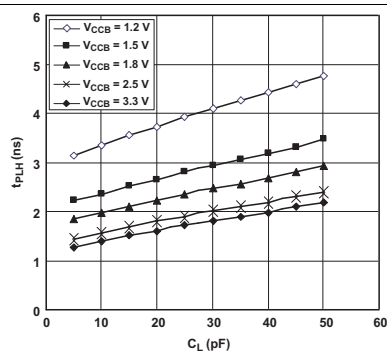
Figure 3. Typical A-to-B Propagation Delay, Low to High
