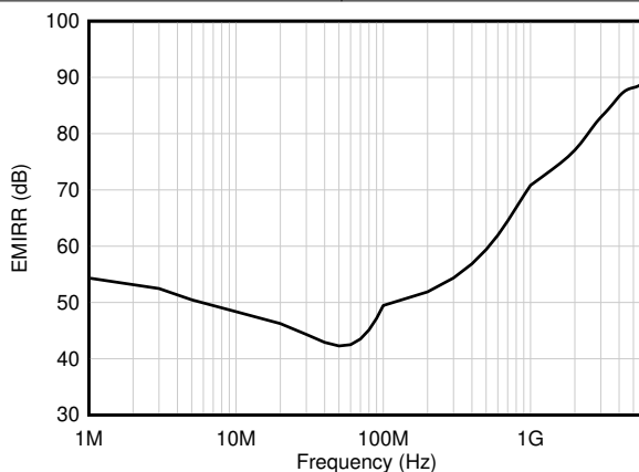
图 6-47. EMIRR (Electromagnetic Interference Rejection Ratio) vs Frequency
