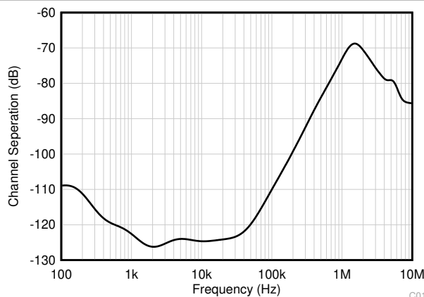
图 6-46. Channel Separation vs Frequency
