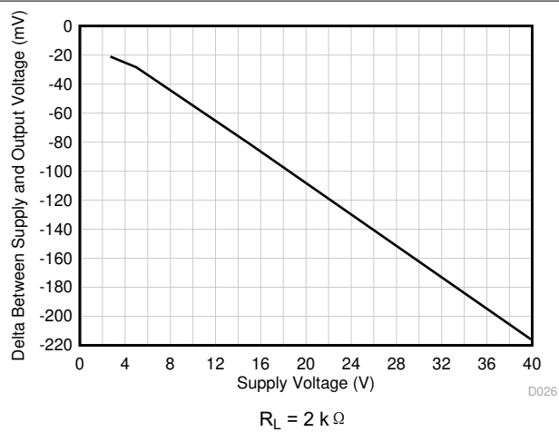
图 6-30. Output Swing vs Supply Voltage, Negative Swing
