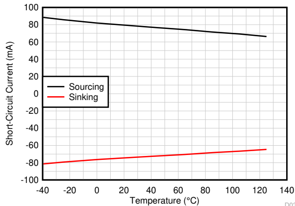
图 6-44. Short-Circuit Current vs Temperature
