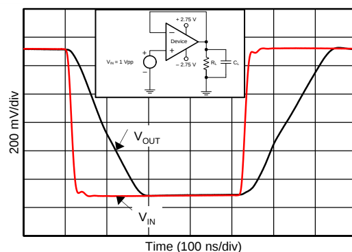
Figure 28. 负过载恢复
