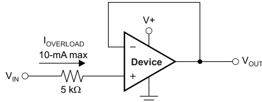
Figure 37. 输入电流保护
