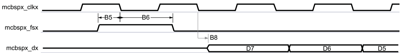
Figure 6-42. McBSP Falling Edge Transmit Timing in Master Mode
