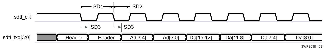
Figure 6-81. SDTI—Single-Edge Mode
