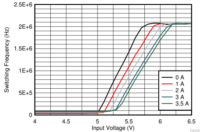
图 8-12. Frequency Dropout Characteristics ( V_{OUT} = 5 V)
