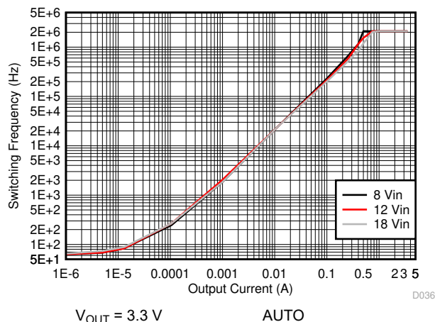
图 9-27. Switching Frequency vs Load Current
