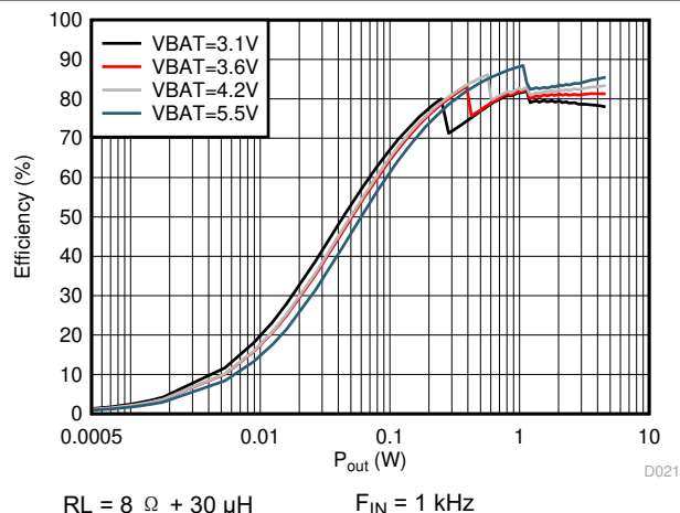
图 6-28. Efficiency vs Output Power
