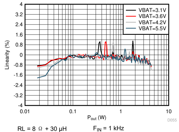
图 6-54. V/I-sense Linearity vs Output Power
