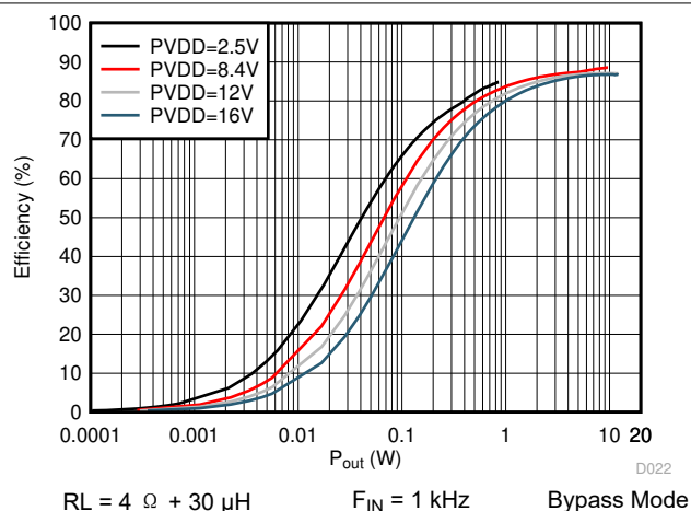
图 6-29. Efficiency vs Output Power
