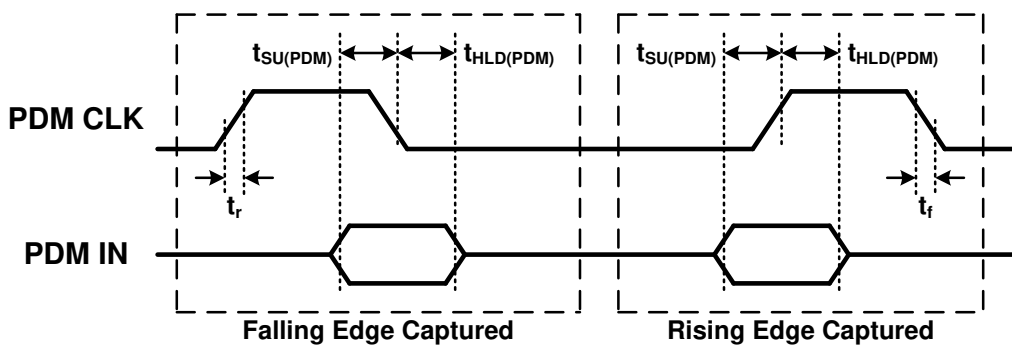
图 6-3. PDM Timing Diagram
