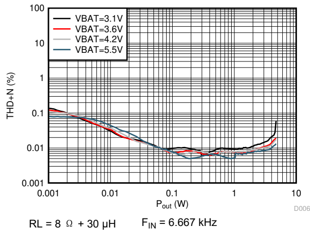
图 6-13. THD+N vs Output Power (DSBGA Package)
