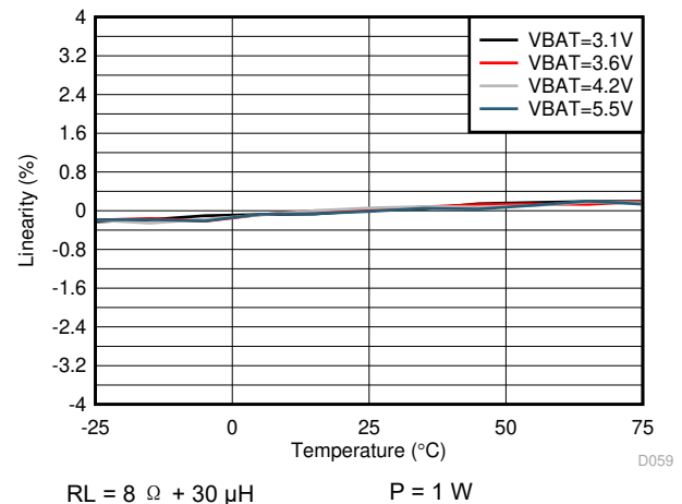
图 6-56. V-sense Linearity vs Temperature
