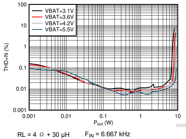
图 6-11. THD+N vs Output Power (DSBGA Package)
