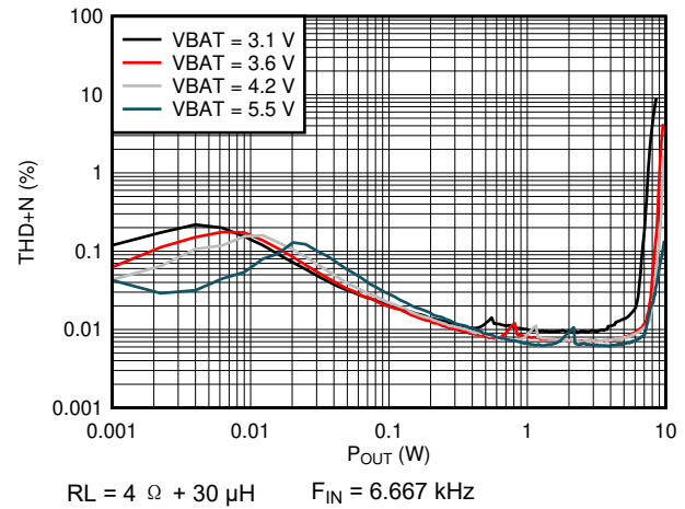
图 6-12. THD+N vs Output Power (QFN Package)
