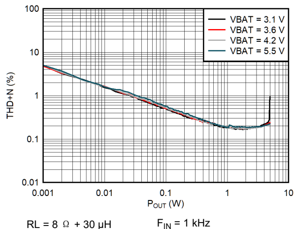
图 6-40. I-sense THD+N vs Output Power (QFN Package)
