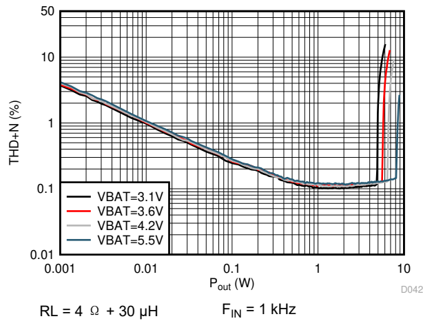
图 6-47. V-sense THD+N vs Output Power
