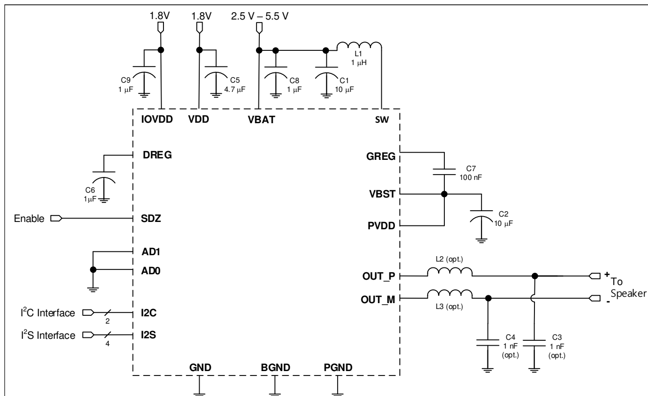
图 9-1. Typical Application - Digital Audio Input with 1S Battery Supply
