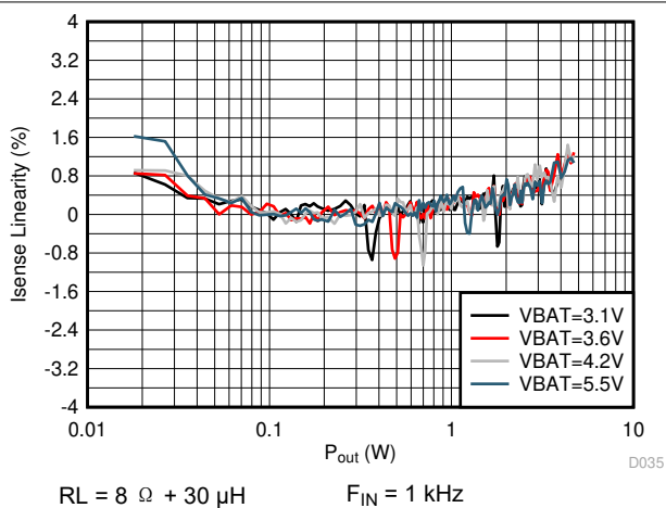
图 6-42. I-sense Linearity vs Output Power
