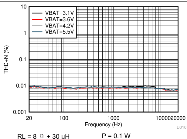
图 6-18. THD+N vs Frequency
