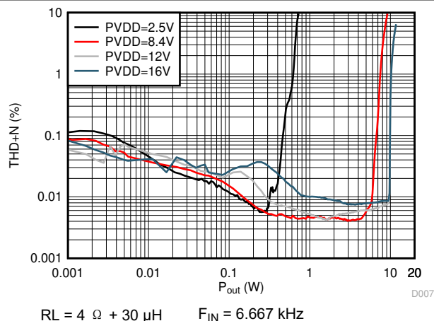
图 6-15. THD+N vs Output Power
