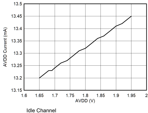
图 6-35. AVDD Idle Current vs AVDD (QFN Package)
