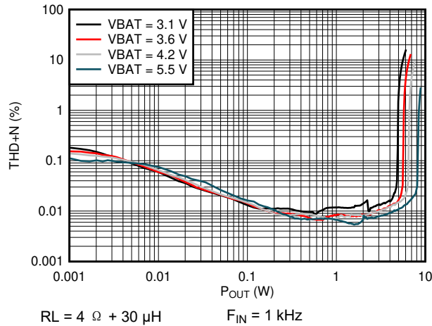
图 6-5. THD+N vs Output Power (DSBGA Package)
