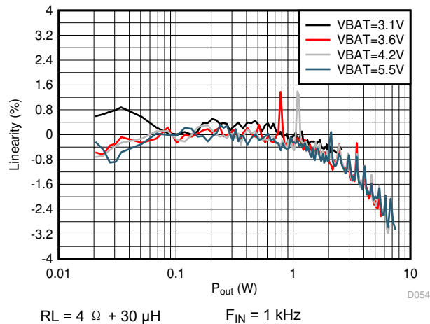
图 6-53. V/I-sense Linearity vs Output Power
