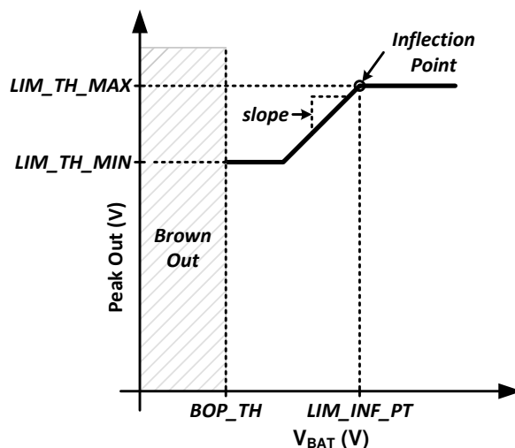
图 8-17. Limiter with Inflection Point and Minimum Threshold
