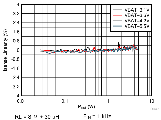
图 6-50. V-sense Linearity vs Output Power
