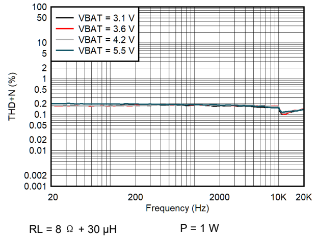
图 6-46. I-sense THD+N vs Frequency (QFN Package)
