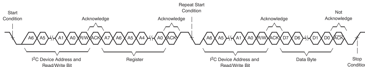
图 8-8. Single-Byte Read Transfer
