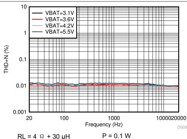
图 6-17. THD+N vs Frequency
