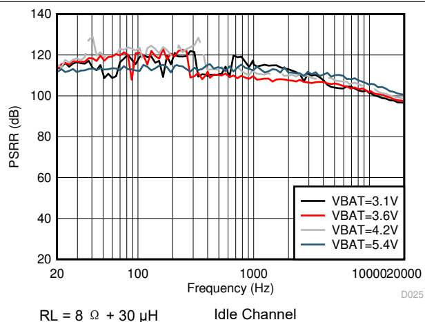
图 6-32. VBAT PSRR vs Frequency
