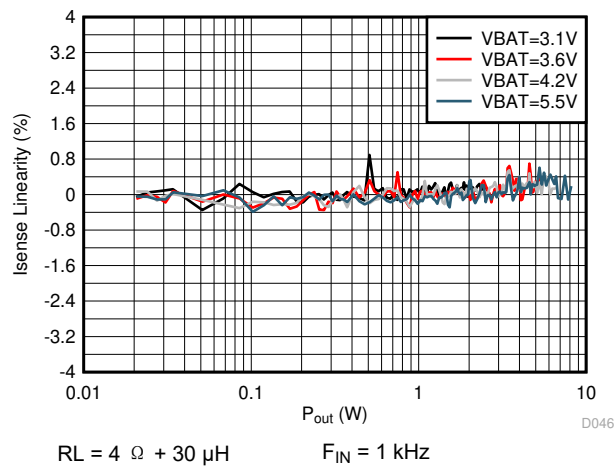
图 6-49. V-sense Linearity vs Output Power
