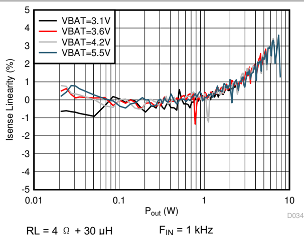
图 6-41. I-sense Linearity vs Output Power
