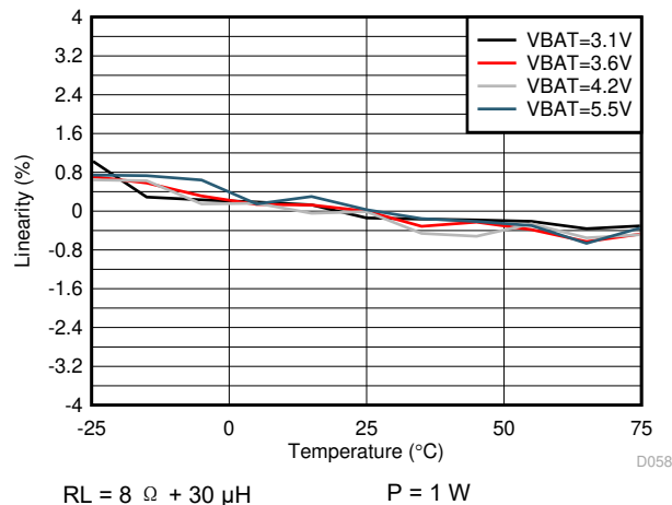
图 6-55. I-sense Linearity vs Temperature
