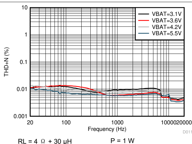
图 6-19. THD+N vs Frequency
