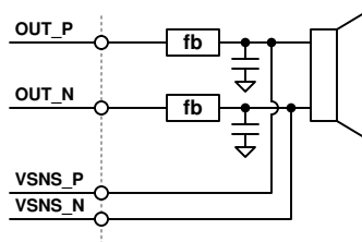
图 8-20. V-Sense Connections
