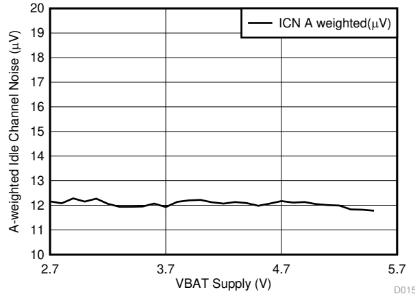
图 6-21. Idle Channel Noise (A-Weighted) vs VBAT
