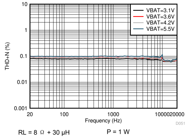
图 6-52. V-sense THD+N vs Frequency
