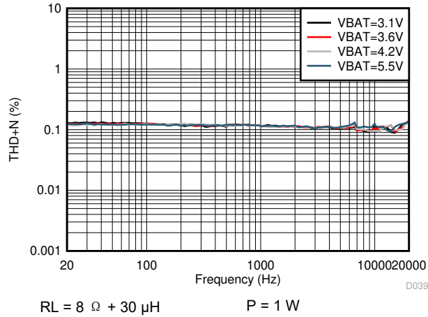
图 6-45. I-sense THD+N vs Frequency (DSBGA Package)
