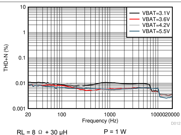
图 6-20. THD+N vs Frequency
