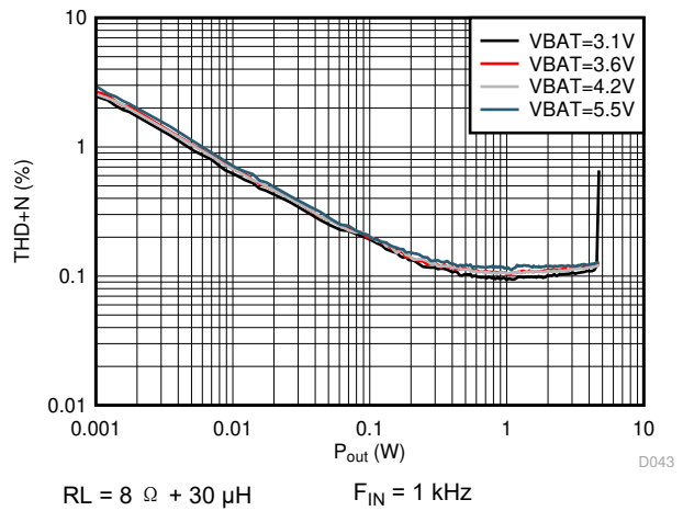
图 6-48. V-sense THD+N vs Output Power
