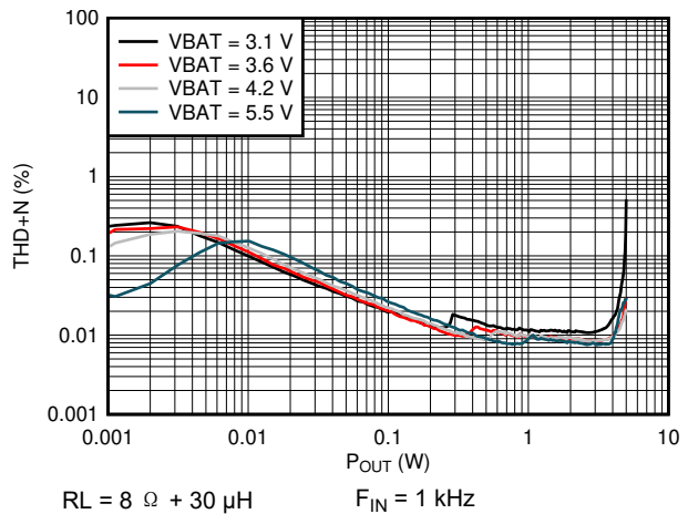
图 6-8. THD+N vs Output Power (QFN Package)
