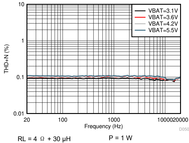
图 6-51. V-sense THD+N vs Frequency
