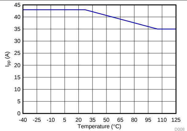
图 8. Max Surge Current (8/20 \mu s) vs Temperature
