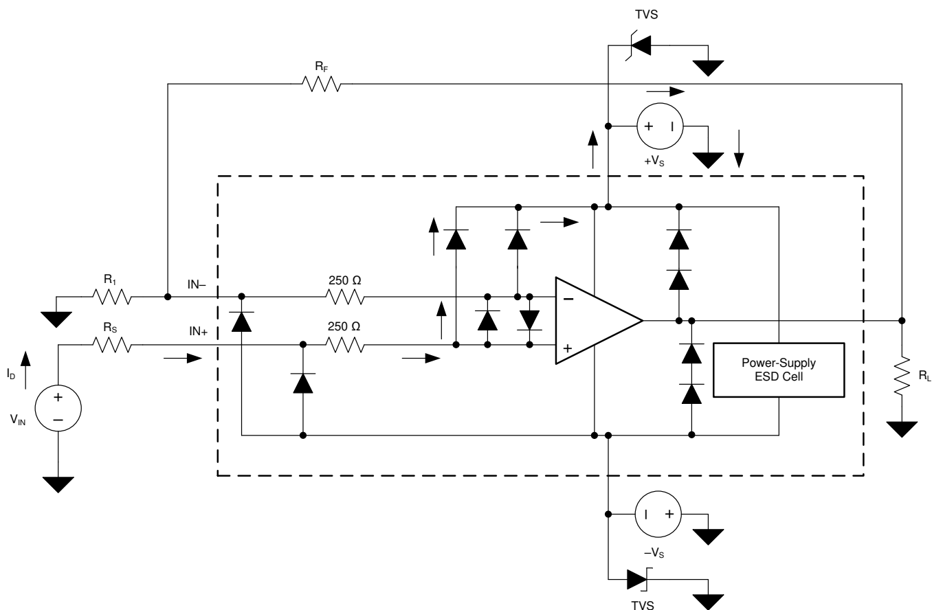
图 43. Equivalent Internal ESD Circuitry Relative to a Typical Circuit Application
