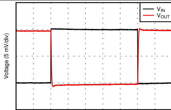
图 33. Positive Overload Recovery
