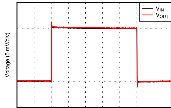
图 32. Negative Overload Recovery
