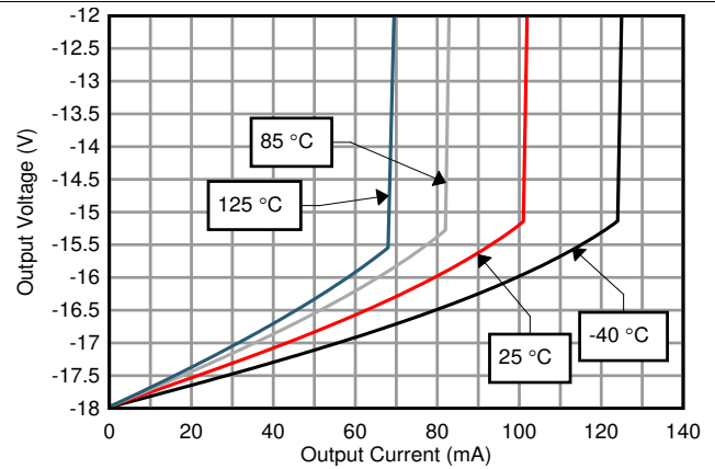
图 26. Negative Output Voltage vs Output Current
