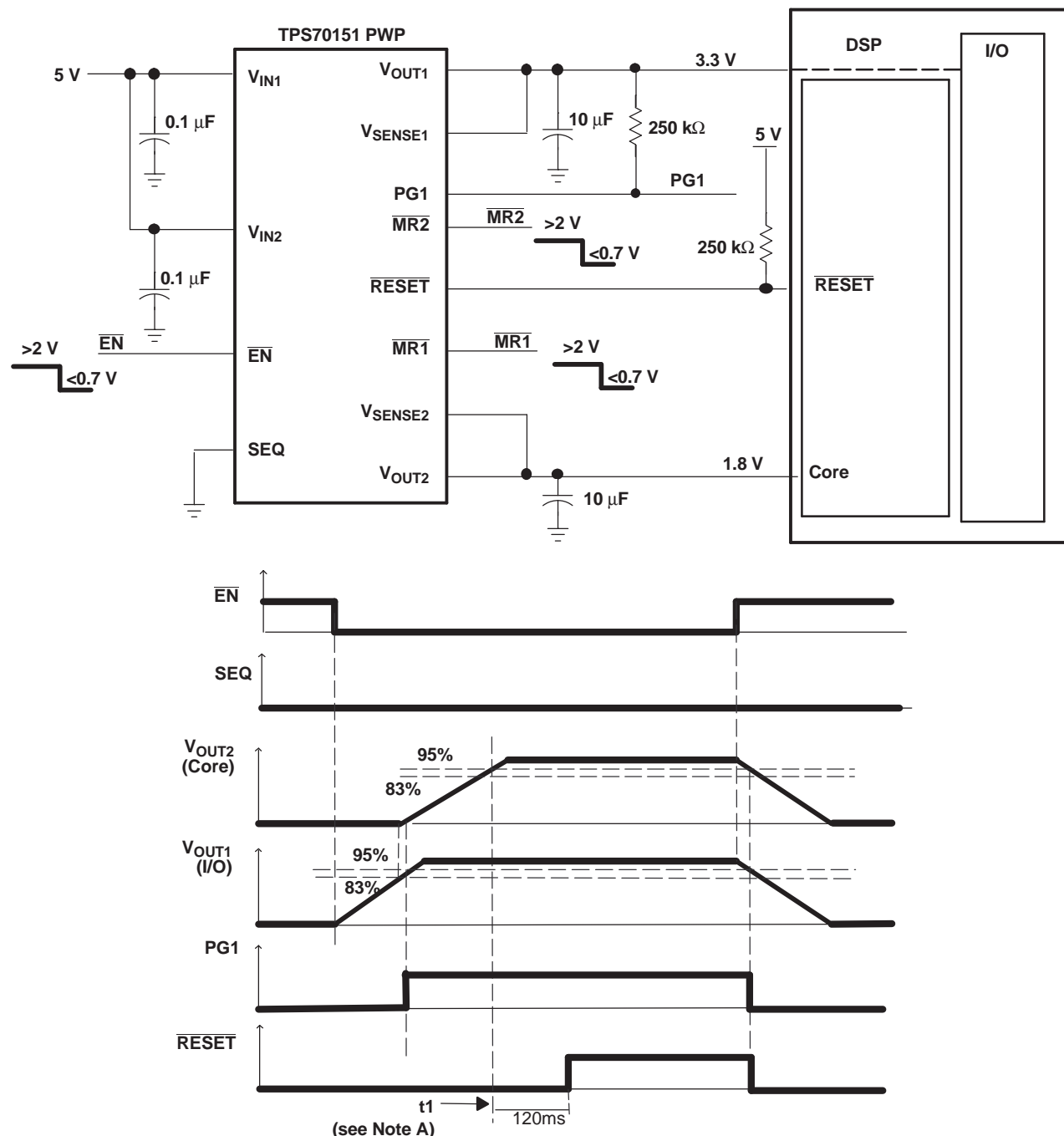
Figure 45. Application Timing Diagram (SEQ = Low)
