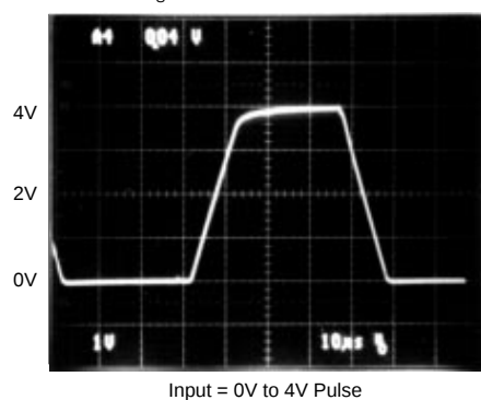
LARGE SIGNAL TRANSIENT RESPONSE V_S = 5V/0V, G = +1, \text{No Load}
