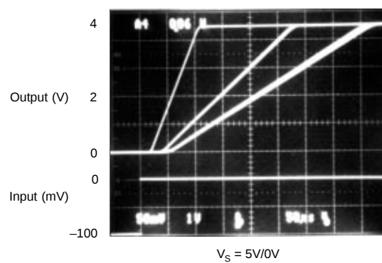
COMPARATOR RISE RESPONSE TIME 10mV, 5mV, 2mV Overdrives
