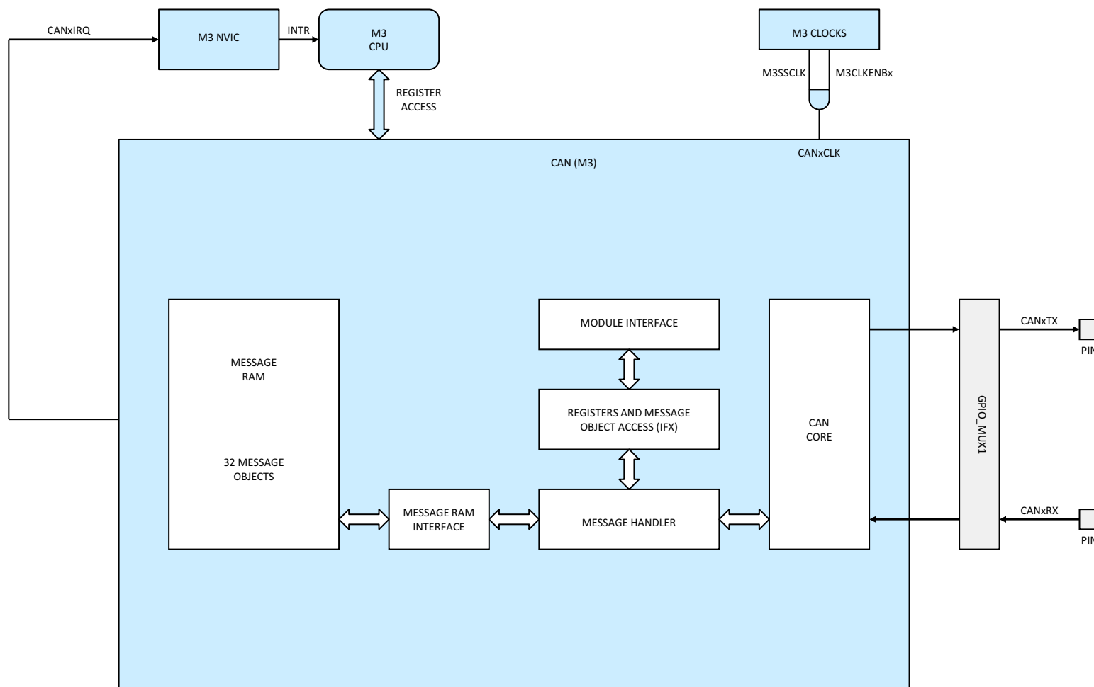
Figure 5-34. CAN (Cortex-M3)
