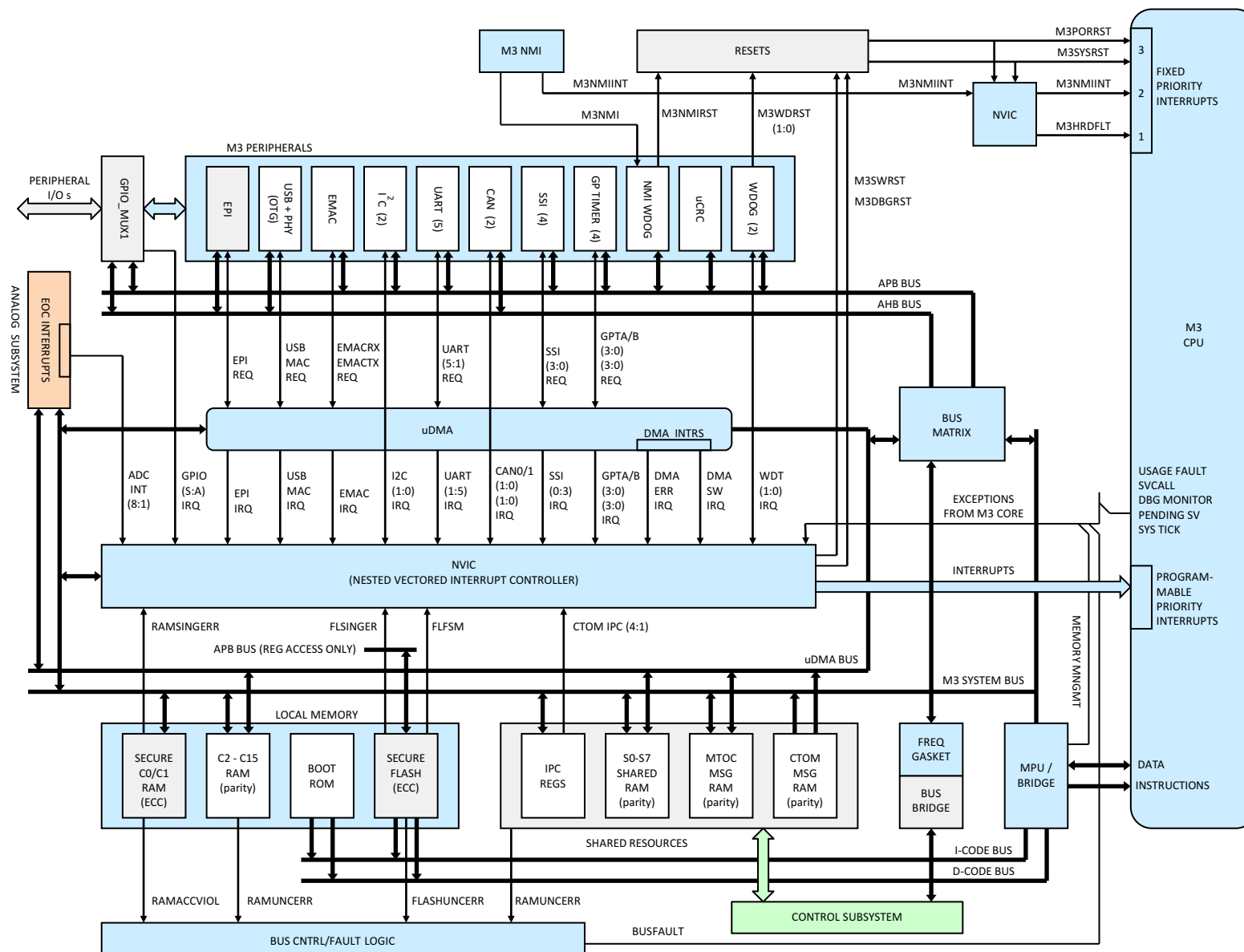
Figure 6-1. Master Subsystem
