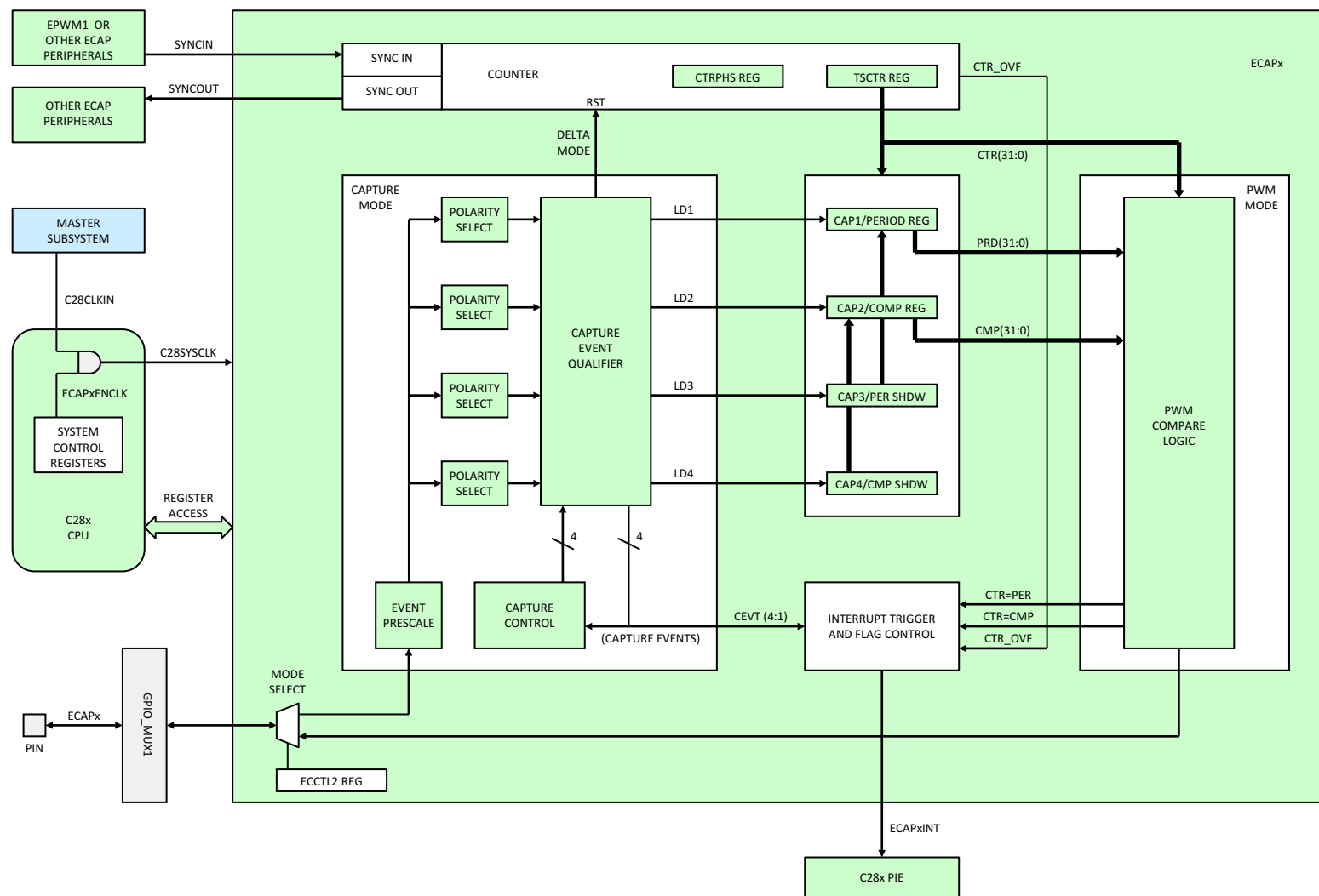
Figure 5-47. eCAP
