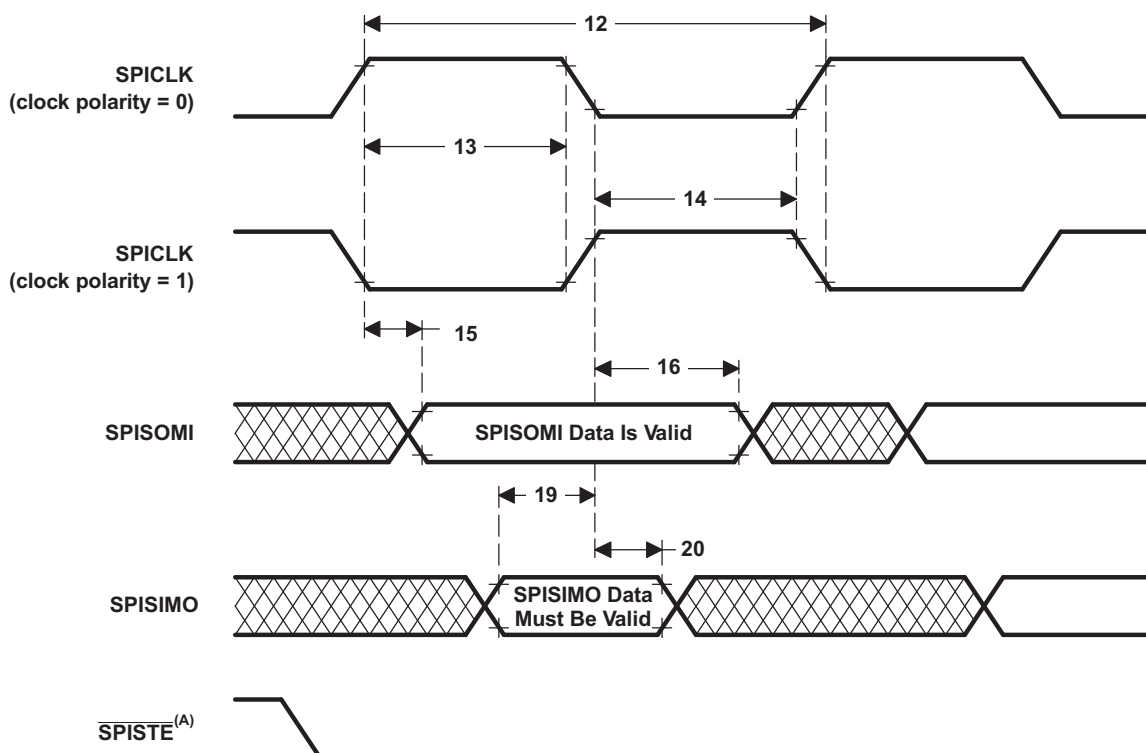
Figure 5-54. SPI Slave Mode External Timing (Clock Phase = 0)
