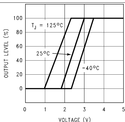
Figure 13. Soft-Start
