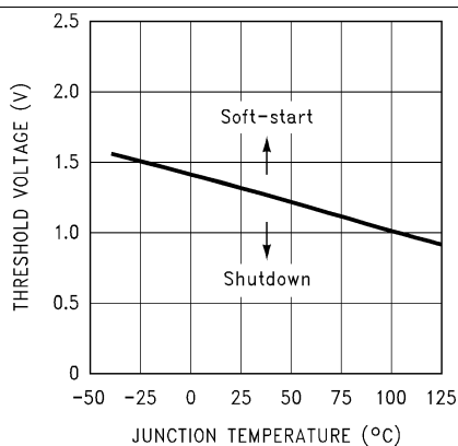
Figure 18. Shutdown/Soft-Start Threshold Voltage
