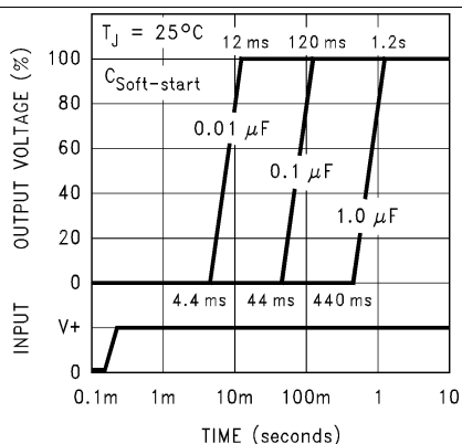
Figure 17. Soft-Start Response
