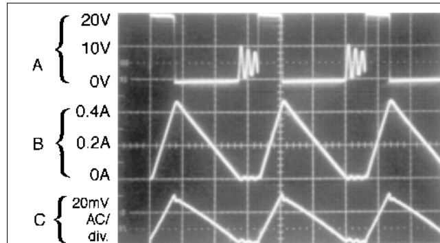
Discontinuous mode switching waveforms V_{IN} = 20\text{ V} , V_{OUT} = 5\text{ V} , I_{LOAD} = 200\text{ mA} L = 33\text{ }\mu\text{H} , C_{OUT} = 220\text{ }\mu\text{F} , C_{OUT}\text{ ESR} = 60\text{ m}\Omega A: Output pin voltage, 10 V/div. B: Inductor current, 0.2 A/div. C: Output ripple voltage, 20 mV/div.
