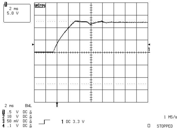
Figure 10-10. Output Voltage Behavior at Full Load Start-up (5 V/div)
