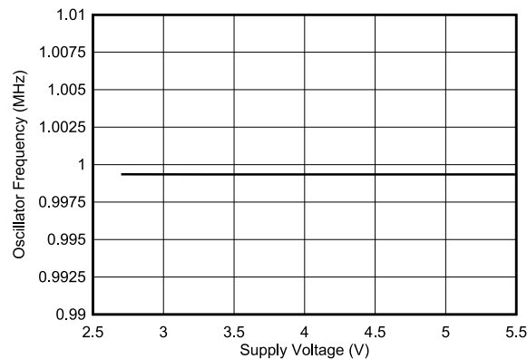
Figure 6-24. Internal Clock Frequency vs. Power Supply
