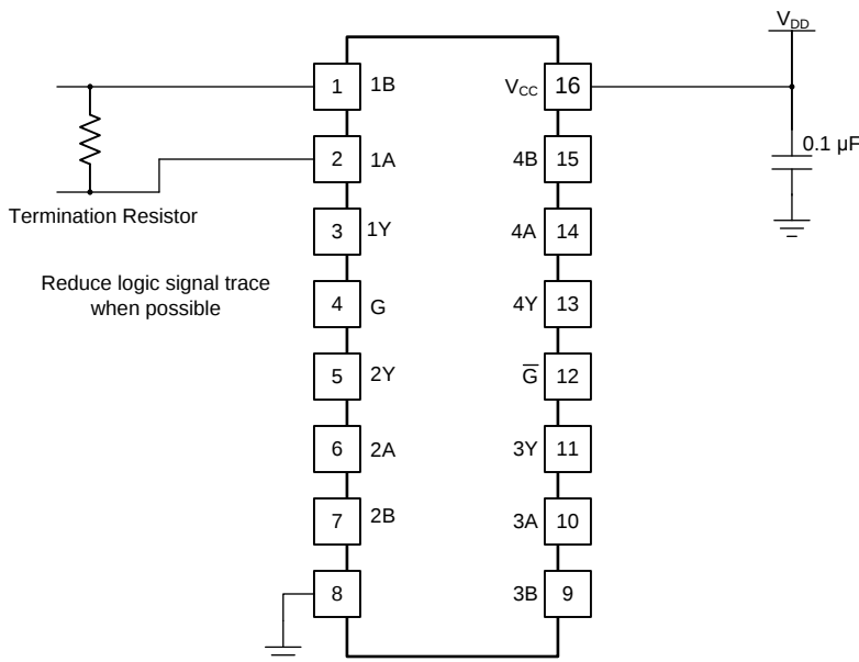
Figure 21. Layout With PCB Recommendations
