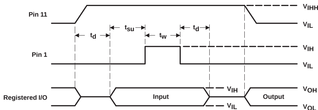
Figure 1. Preload Waveforms
